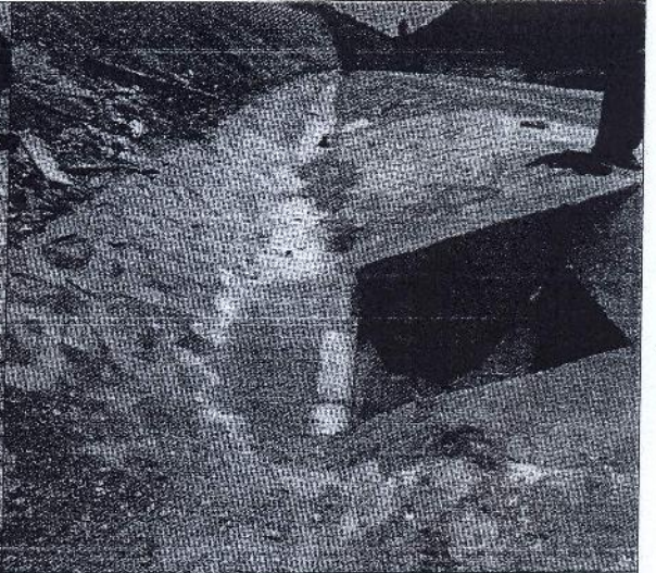
Km 47+220 LHS. Lowering of ditch lining at relief culvert drop-inlet and repair of stone pitching.
